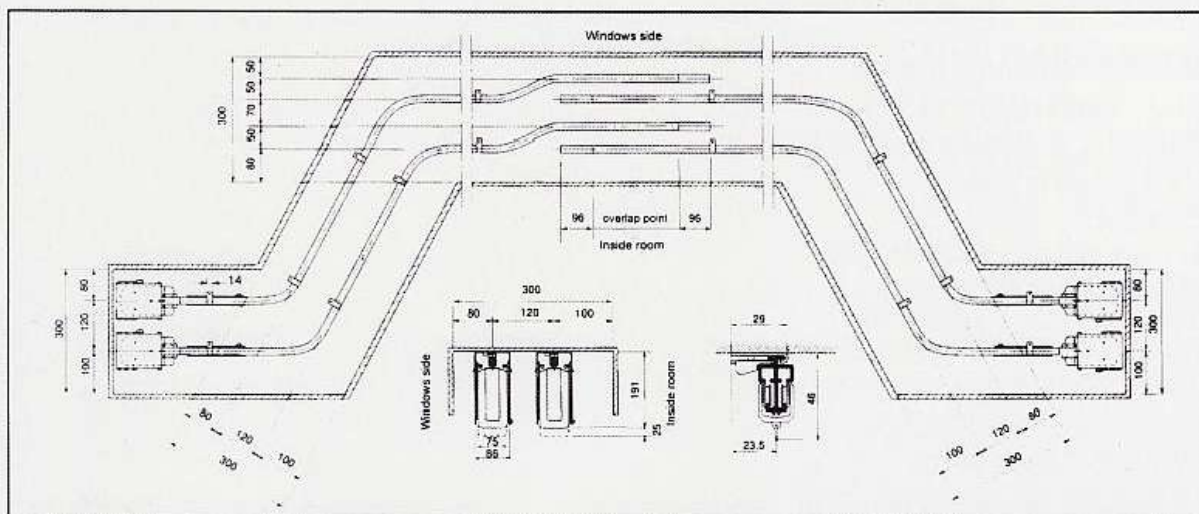
“拱型” Arcaded shape
