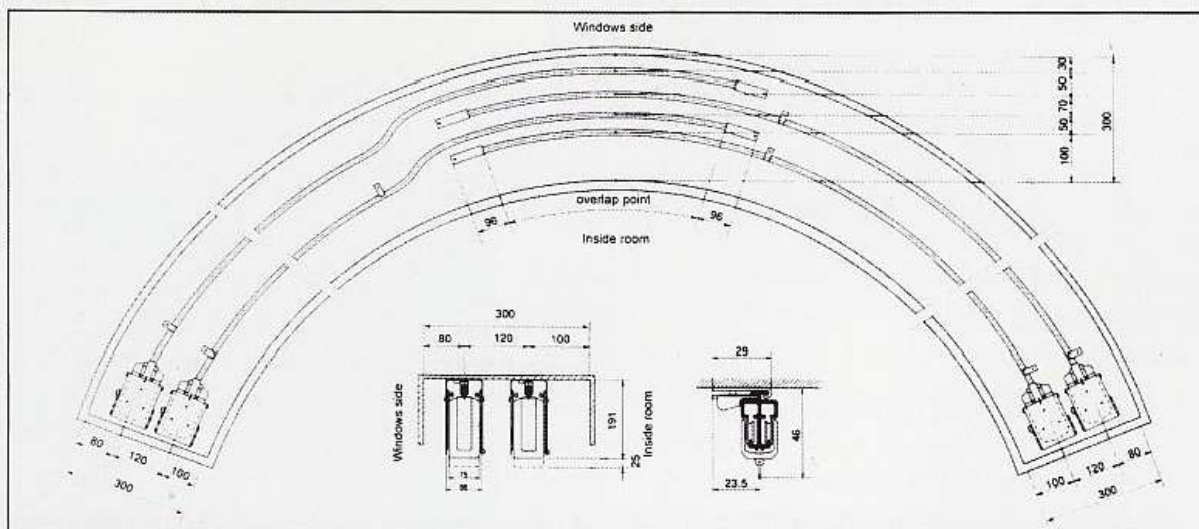
“圓弧型” Dome shape
